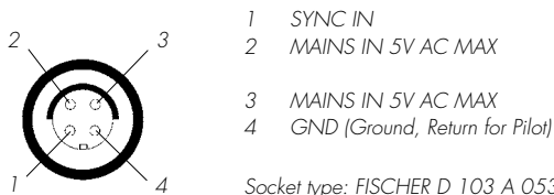
SYNC BOX SYNC IN (female) Top View
