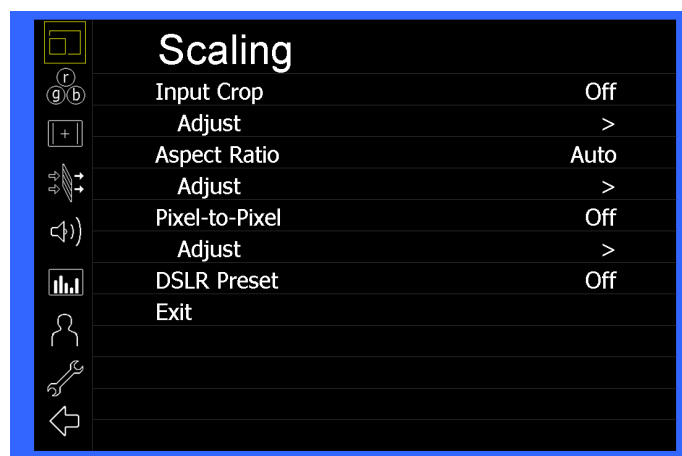
Scaling Submenu
