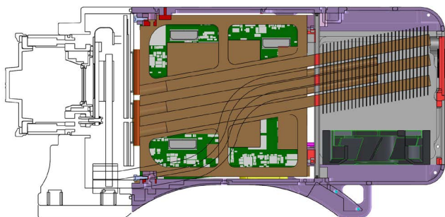
2009. Cooling design.
