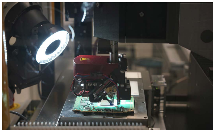
Wire bonding
