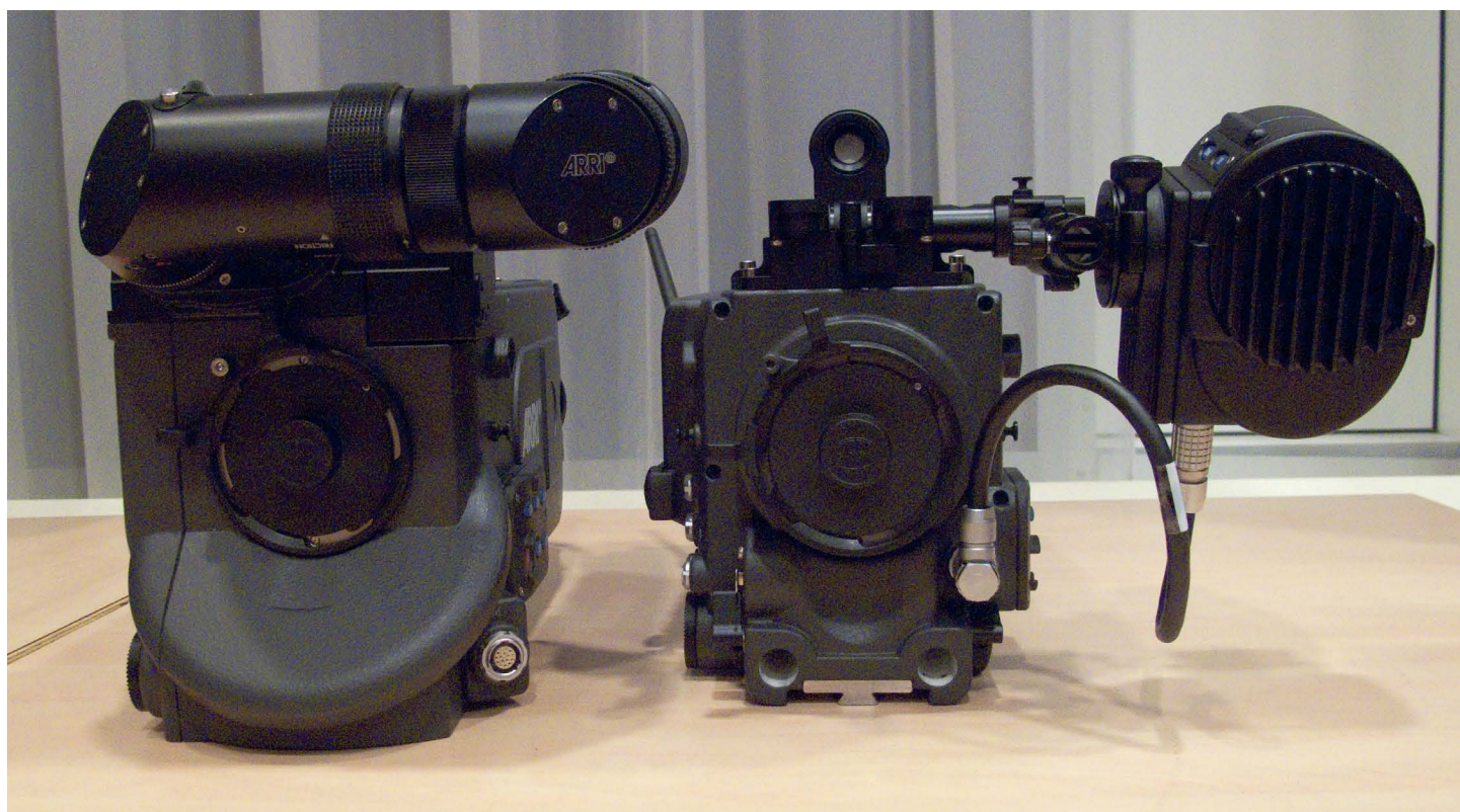
Above: front view of Alexa EV pre-prototype with electronic finder, and lightweight 15mm supports under PL mount.
